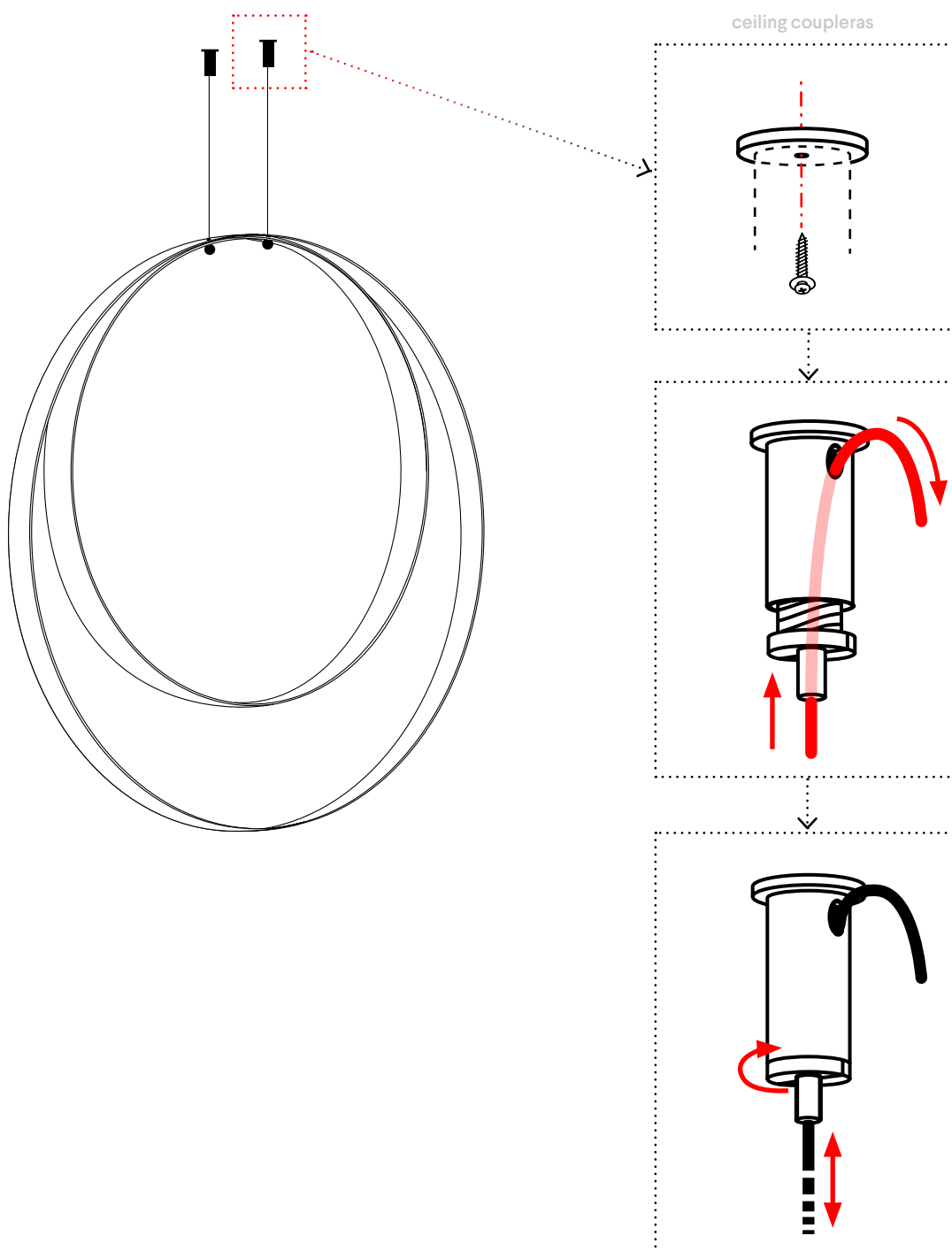
2X Galvanized cable with ball tips (Provided and fixed to the products)
